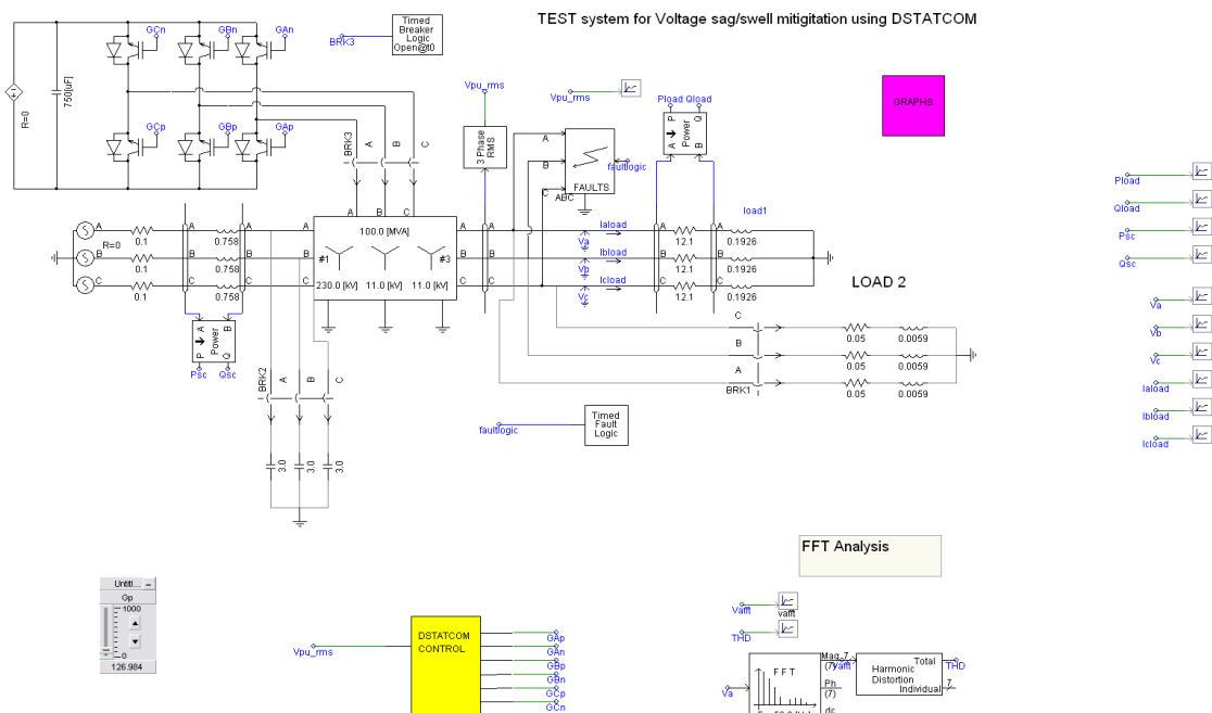
Fig.4 (a) PCSAD/EMTDC model of a three phase 6-pulse. Fig.4 (b) Control circuit of D-STATCOM
