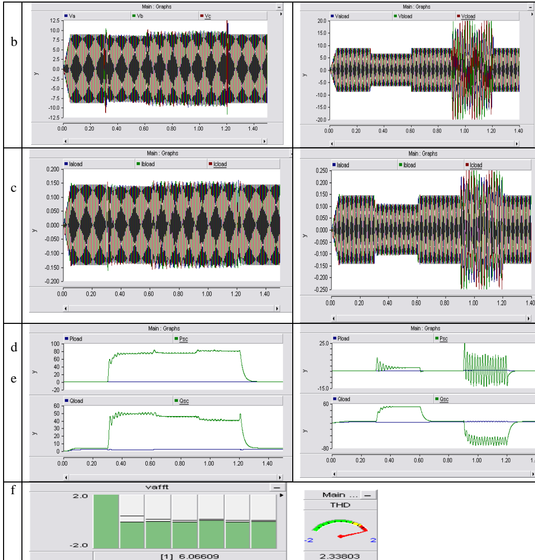
Fig.7 waveforms due to load switching (a) rms load voltage (pu) (b) Instantaneous load voltages(KV) (c) Instantaneous load currents(KA) (d) load and source active powers(MW) (e) load and source reactive power(MVAR) (f) harmonic analysis at load during fault(%)
