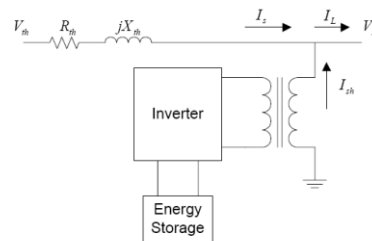
Fig.2 operating modes of the effectiveness of D-STATCOM depends on the source impedance Z_{th} and the fault level.
